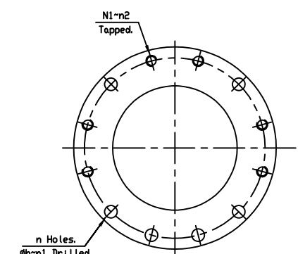
Detail of flange for size 10" (250) only.
