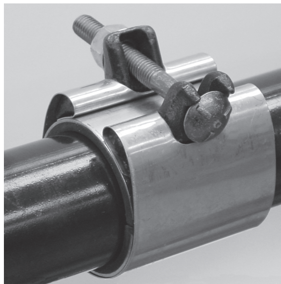
Note: Gasket is shown in proper alignment with stainless steel band.
