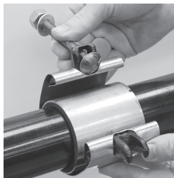
With lugs centered over one of the gap bridges.
