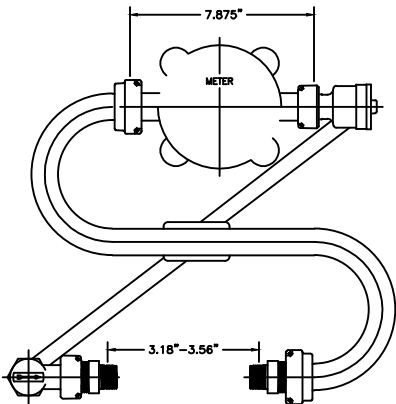
DETAIL OF TANDEM ASS'Y
