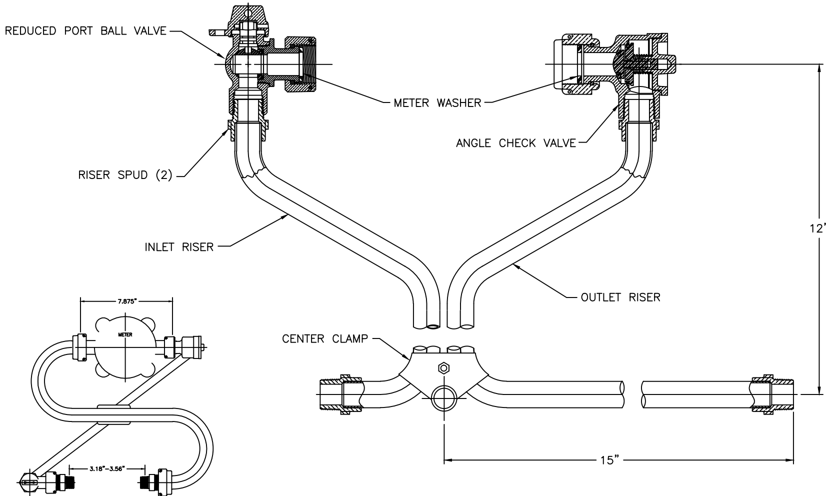
DETAIL OF TANDEM ASS'Y
