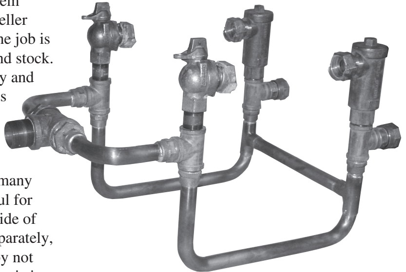
Optional ASSE dual check valves shown
