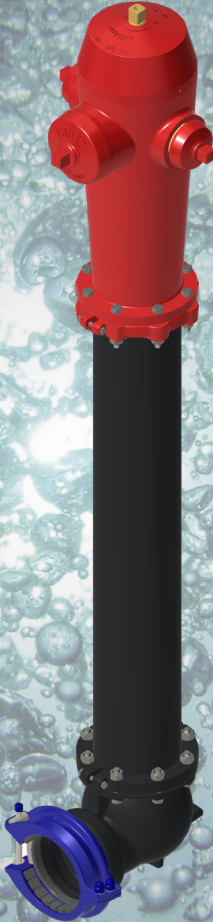
CANADA VALVE™ CENTURY FIRE HYDRANTS: CENTURY | B-50-B
